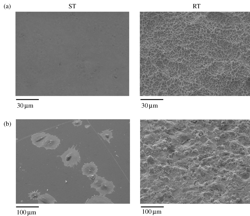
Figure 1 SEM images of the ST and RT surfaces. The surfaces are shown before (a) and after (b) 3 h of incubation with AB cells (magnification \times 750 and \times 200 , respectively).
