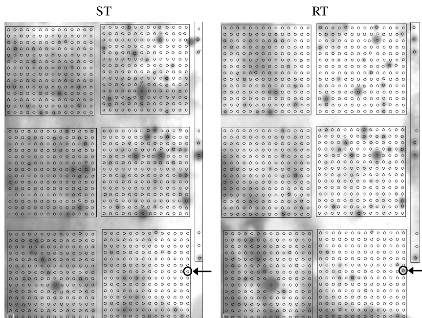
Figure 2 Autoradiograph images of the Atlas ® gene array filters showing the relative hybridisation levels of specific genes from AB cells on ST and RT surfaces, after 3 h incubation. 32 P-labelled dCTP was used to radiolabel cDNA sequences for hybridisation. The arrows show the relative up-regulation of the signal on RT, compared to ST, for the neurotrophin 4 gene.
